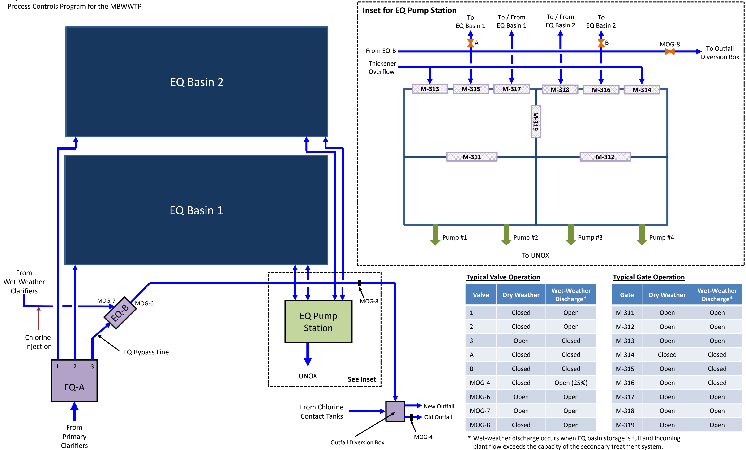
Figure 2-3 Equalization Flow Schematic
