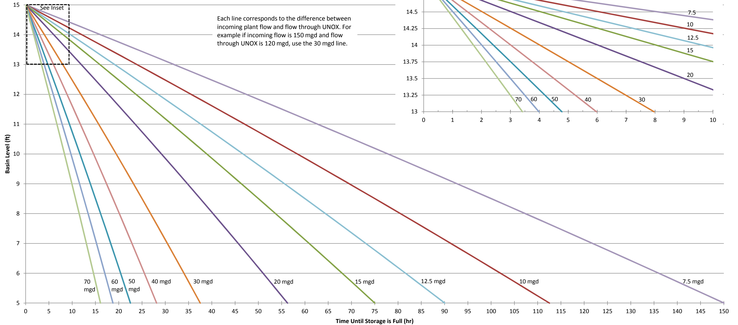
Figure 2-4 Relationships Between Flow, Basin Level, and Remaining Storage
